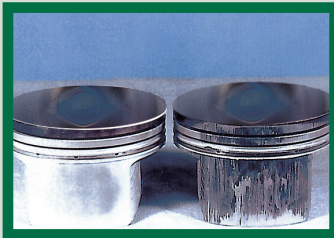
Piston and Piston Ring Scuffing
