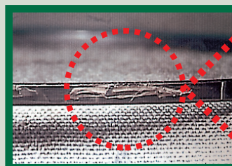
Coating Flaking of Piston Ring Running Face
